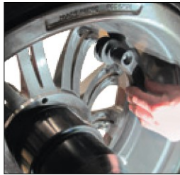
Automatic programs.
